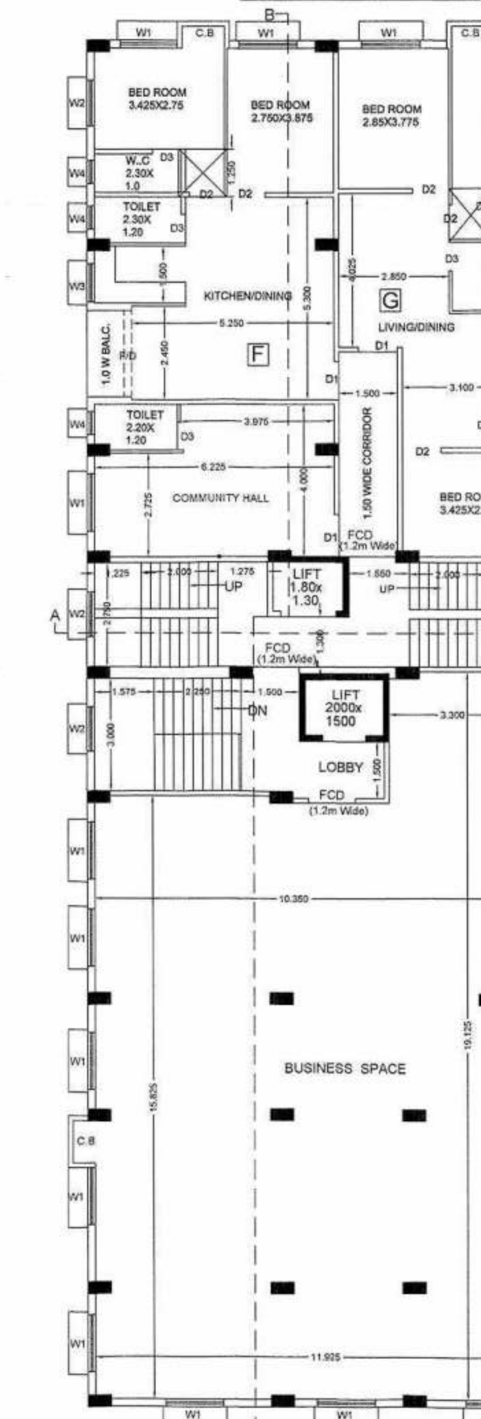
FLOOR-01 1ST FLOOR PLAN
